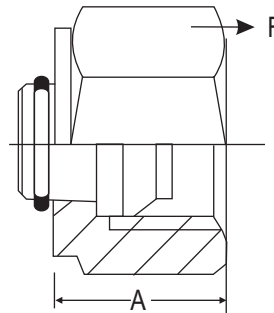
Dimensional Details :
